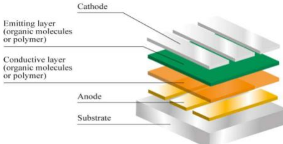
Figure 1: Fundamental Structure of OLED
