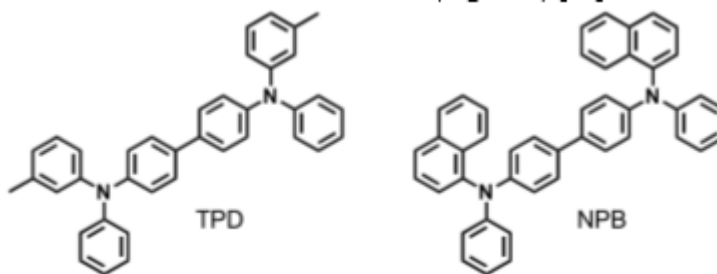
Figure 5 : Commonly used components in holes transport layer.
