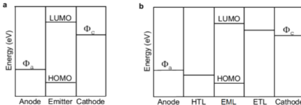
Figure 6: Energy-level diagrams of (a) a single-layer OLED and (b) a multilayer OLED with a hole transporting layer (HTL) and an electron transporting layer (ETL) sandwiching an emissive layer (EML).
