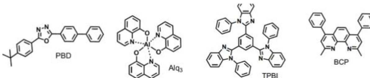
Figure 4 : Commonly used components in electrons transport layer
