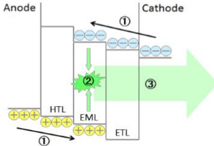
Figure 2: Scheme of the electroluminescence mechanism in an OLED.
