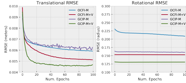
Fig. 4 RMSE of Mean Post-Grasp Object Displacement Predictions for Variants of GDN on the Validation Set During Training We observe that models that incorporate displacement variance prediction consistently outperform ones that do not, and GDN on image patches outperforms operating on the full image.
