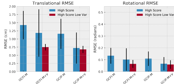
Fig. 7 Real World Translational and Rotational RMSE of Grasp Displacement Predictions.
