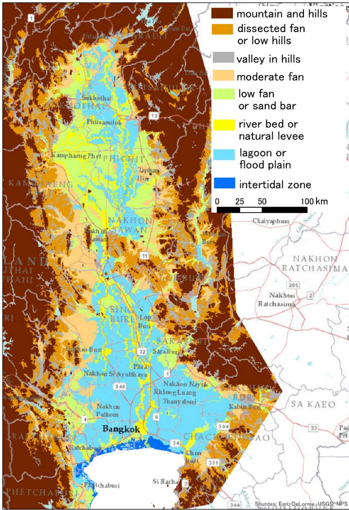
Figure 3. Terrain classification of the Central Plain of Thailand using HAND and slope gradient calculated using a 90 m DEM interpolated from MERIT. The legend was designed according to the existing manual geomorphological map [5] .
