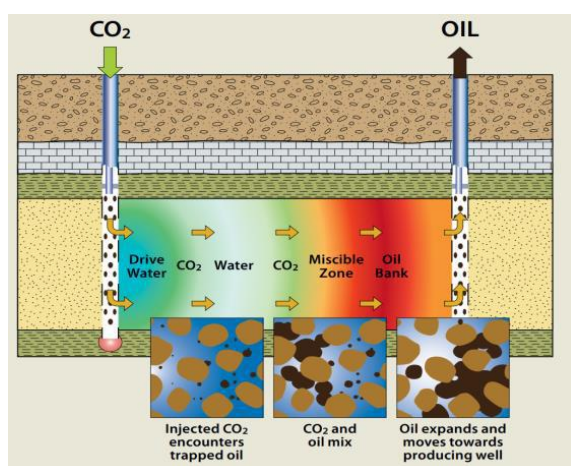
Figure 1: The diagram of CO 2 WAG process (E. Halland et al., 2012).
