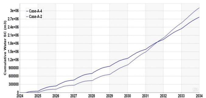
Figure 21: Cumulative water production without AICV for the horizontal case (A-2) and the vertical case (A-4).
