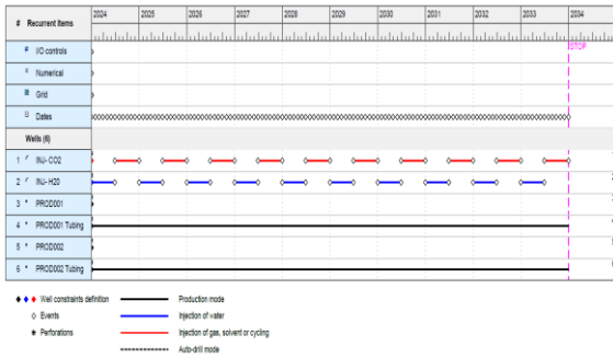
Figure 7: The timeline of the WAG cycle periods.
