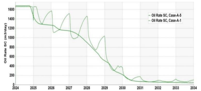
Figure 10: The field oil rate of the two producer wells at standard condition for case-A-1 and case-A-5.
