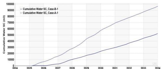
Figure 16: The field cumulative water at standard condition for case-A-1 (homogeneous) and case-B-1 (heterogeneous).
