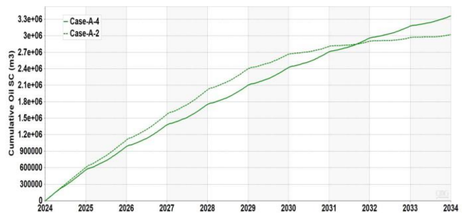
Figure 20: Cumulative oil production without AICV for the horizontal case (A-2) and the vertical case (A-4).
