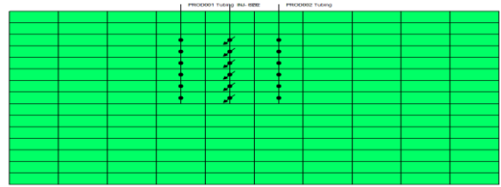
Figure 9: The I-K direction view of the vertical placement of the injector and producer wells.
