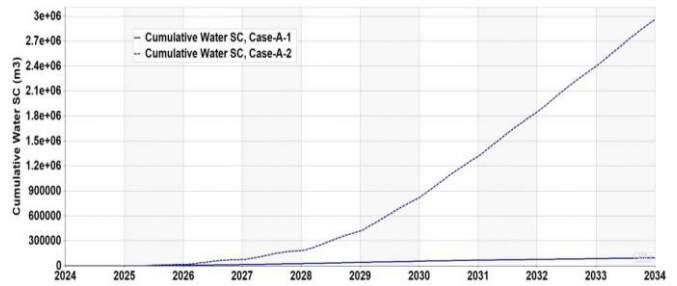
Figure 14: The field cumulative water of the two producer wells at standard condition for case-A-1 and case-A-2.
