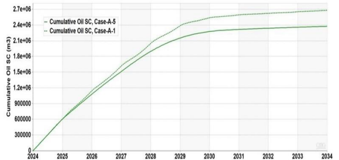
Figure 11: The field cumulative oil of the two producer wells at standard condition for case-A-1 and case-A-5.
