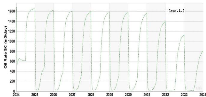
Figure 18: The field oil rate for the modified case-A-2 with less well spacing distance.
