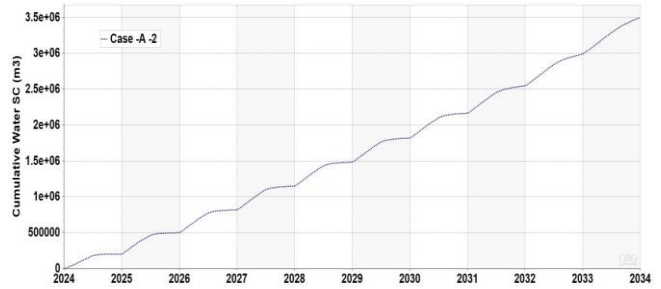
Figure 19: The field cumulative water volume for the modified case-A-2 with less well spacing distance.
