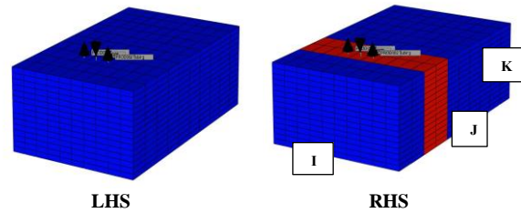
Figure 6: The 3-D view of the homogeneous (LHS) and heterogeneous reservoir (RHS).
