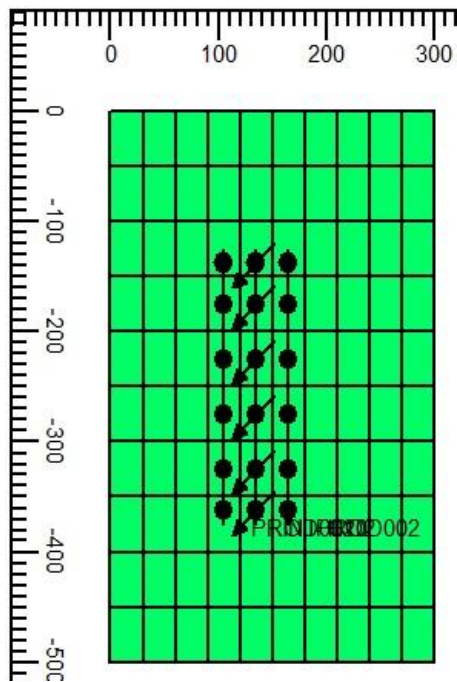
Figure 17: The modified case-A-2 with less well spacing distances.
