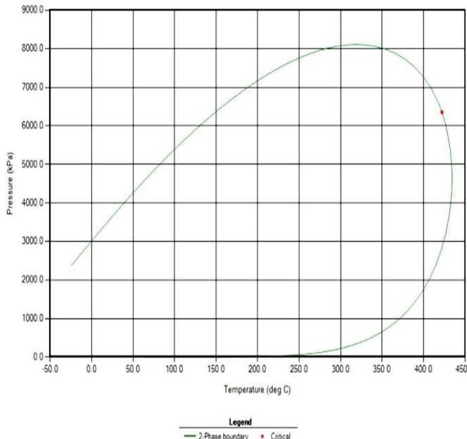
Figure 5: The P-T phase envelope of CO 2 created in WinProp.
