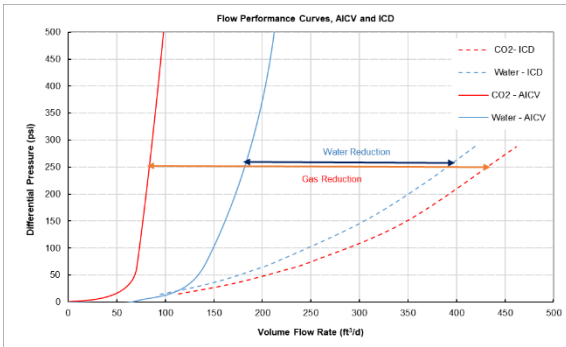
Figure 4: The performance curves of pressure and volumetric flow rate for AICV and ICD (Taghavi et al., 2023).
