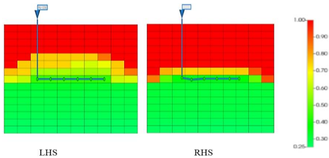
Figure 12: The reservoir oil saturation for the WAG (LHS) and the water injection (RHS).
