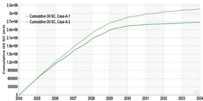
Figure 13: The field cumulative oil of the two producer wells at standard condition for case-A-1 and case-A-2.
