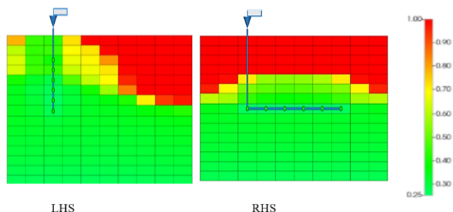
Figure 22: The oil saturation at year 2034 of case-A-4 and case-A-1 for the vertical (LHS) and horizontal (RHS) CO 2 injection.
