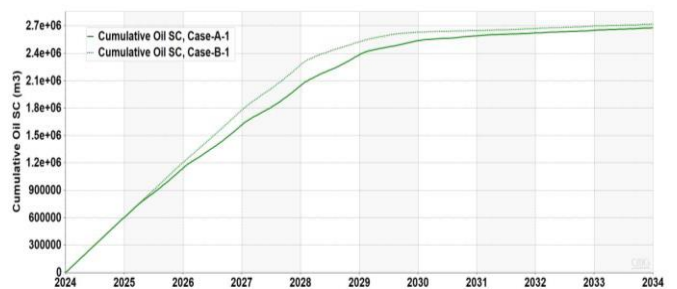
Figure 15: The field cumulative oil at standard condition for case-A-1 (homogeneous) and case-B-1 (heterogeneous).
