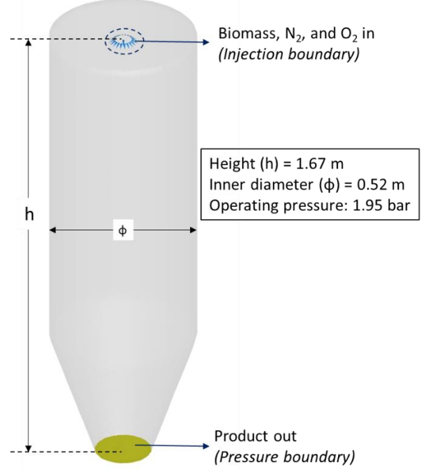
Figure 2: Boundary conditions
