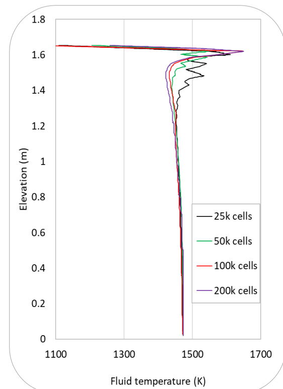
Figure 4: fluid temperature versus elevation. The fluid temperature is radially averaged.
