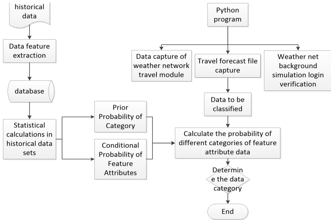
figure 1 Naive Bayes algorithm classification process
