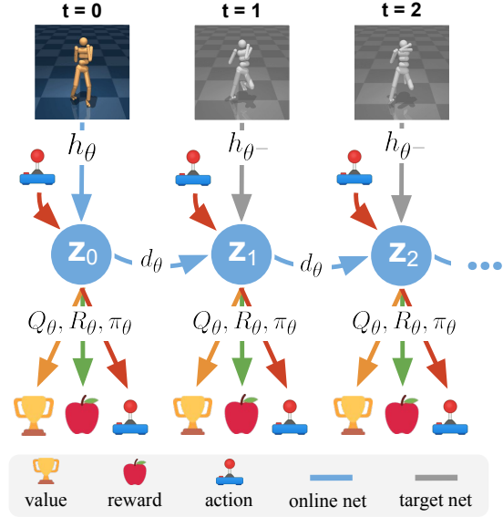
Figure 2. Training our TOLD model. A trajectory \Gamma_{0:H} of length H is sampled from a replay buffer, and the first observation \mathbf{s}_0 is encoded by h_\theta into a latent representation \mathbf{z}_0 . Then, TOLD recurrently predicts the following latent states \mathbf{z}_1, \mathbf{z}_2, \dots, \mathbf{z}_H , as well as a value \hat{q} , reward \hat{r} , and action \hat{\mathbf{a}} for each latent state, and we optimize TOLD using Equation 7. Subsequent observations are encoded using target net h_{\theta^-} ( \theta^- : slow-moving average of \theta ) and used as latent targets only during training (illustrated in gray).
