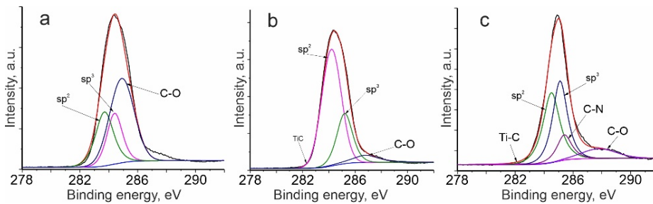
Fig. 1. XPS spectra of C1s coatings: a – Ti/TiN/a-C, b – Ti/TiN/a-C:Ti, c – Ti/TiN/a-C:Ti:N
