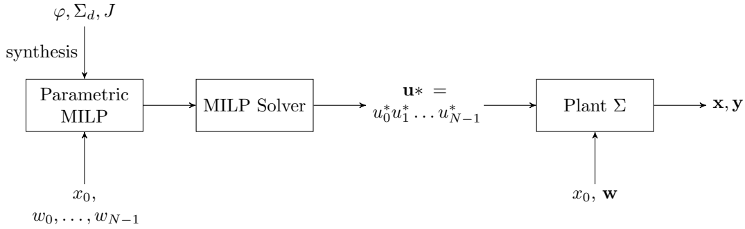
Figure 1: Open Loop Scenario. A parametric Mixed-Integer Linear Program is generated from the STL formula \phi , the discrete-time plant model \Sigma_d and the cost function J . The parameters of this MILP are the initial state x_0 and disturbance vector \mathbf{w} . When those are provided, a solver can compute an optimal solution \mathbf{u}^* for horizon N which is passed and used by the plant \Sigma .
